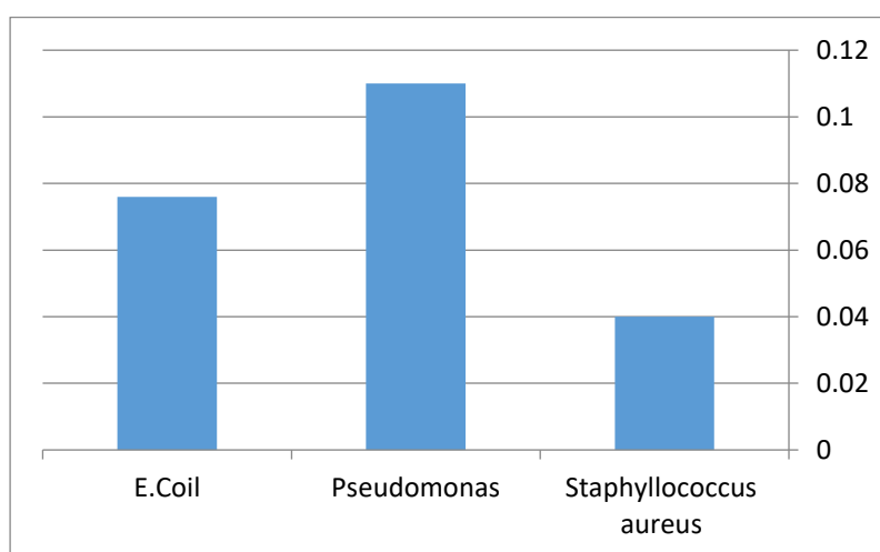
Figure 5. Comparison of antimicrobial activity of cold aqueous extract of menthe leaves with concentration 50% against the bacteria
